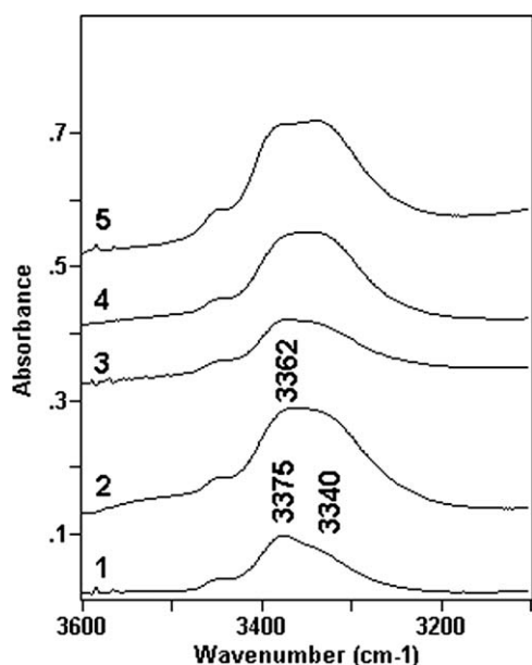
Figure 2 FTIR spectra of \text{PUR}_{\text{PCL}/2} (1), \text{PUR}_{\text{PCL}/3,7} (2), \text{PUR}_{\text{PCL}+\text{a-PHB}/2} (3), \text{PUR}_{\text{PCL}+\text{a-PHB}/3,7} (4), and \text{PUR}_{\text{a-PHB}} (5).
