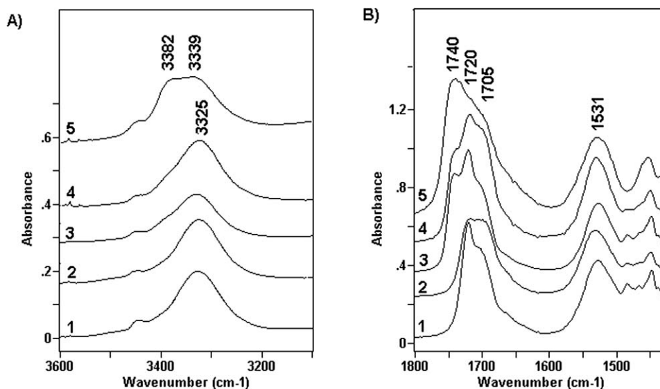
Figure 1 FTIR spectra of \text{PUR}_{\text{PTMO}/2} (1), \text{PUR}_{\text{PTMO}/3,7} (2), \text{PUR}_{\text{PTMO}+\text{a-PHB}/2} (3), \text{PUR}_{\text{PTMO}+\text{a-PHB}/3,7} (4), and \text{PUR}_{\text{a-PHB}} (5).
